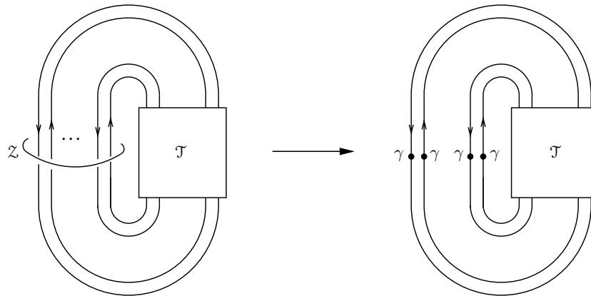
Figure 15: Standard presentation.
