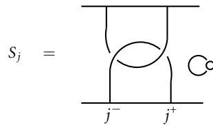
Figure 4: Tangle for S_j .
