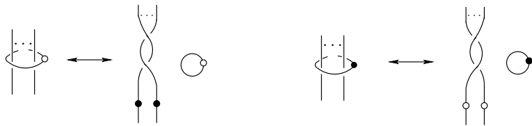
Figure 14: Fenn–Rourke move.
