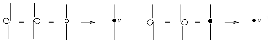
Figure 5: Twist assignments.
