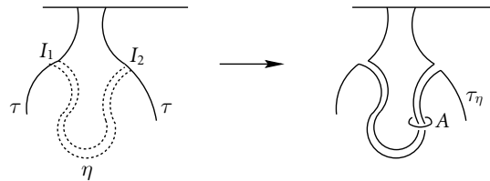
Figure 8: \eta -surgery.
