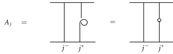
Figure 2: Tangle for A_j .
