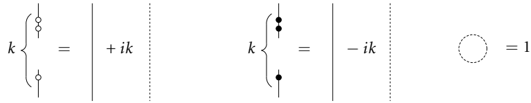
Figure 13: Framing shift.
