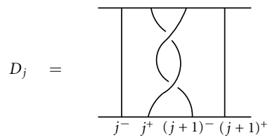
Figure 3: Tangle for D_j .
