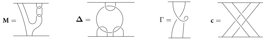
Figure 10: Tangles for multiplications.
