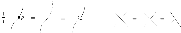
Figure 11: Transparent \rho -decorated strand.
