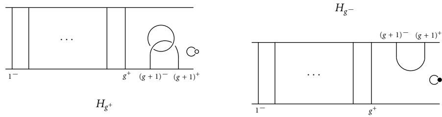
Figure 9: Tangles for Handle additions.
