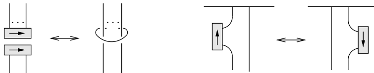
Figure 12: Coupons for 1-handles.
